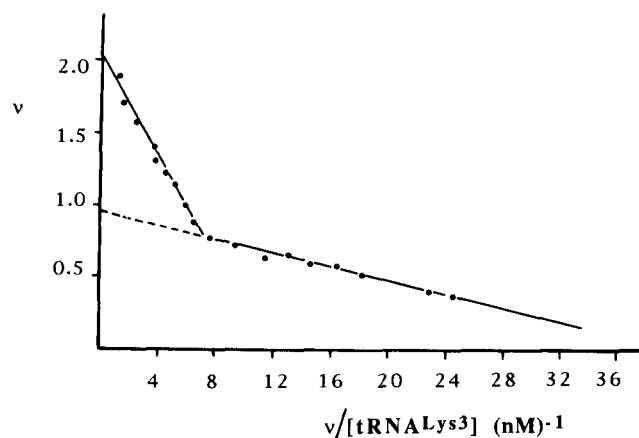
Fig. 1. Determination of K_d values of the complex between HIV-1 RT p66/p51 and tRNA Lys3 using Scatchard plot for the fluorescence data representation.
